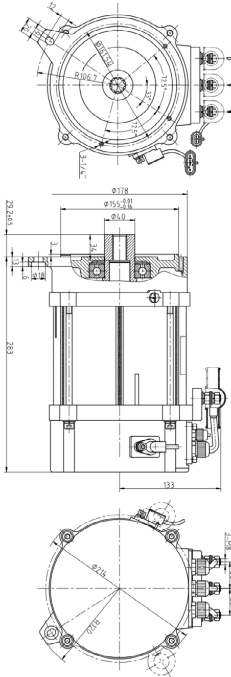
10-000823 5KW AC Motor
